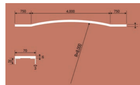
FA-7043 やり投げ用円弧
